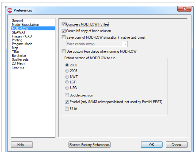
The Preferences dialog showing the MODFLOW tab.
