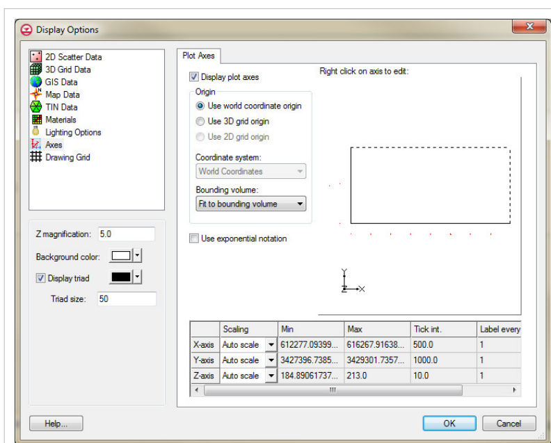
The Display Options dialog showing the Plot Axes tab in GMS 9.2 and earlier.
